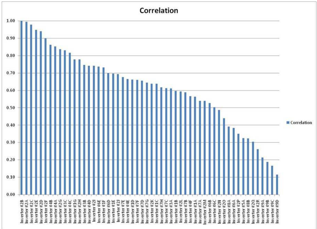
Figure 6. Correlation coefficient of 1-min step changes in power output between different inverters (relative to Inverter #2B) within a 13.2-MW PV plant in the Southwest on a highly variable day.
